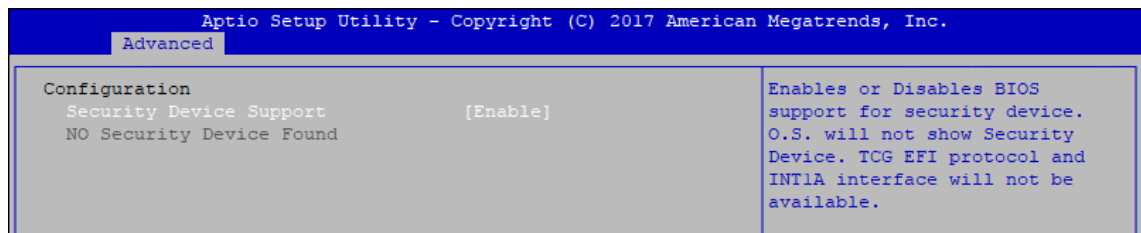
Figure 4-3-4 : Trusted Computing
